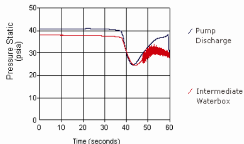
Pump Trip + Discharge Valve Close Case
